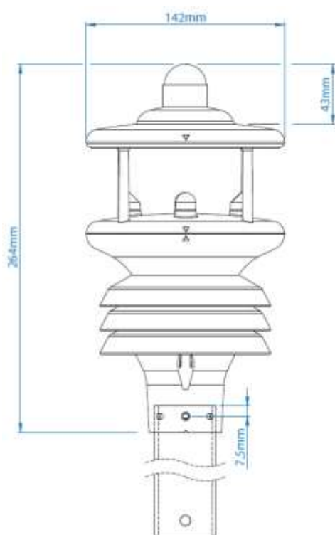
GMX501
