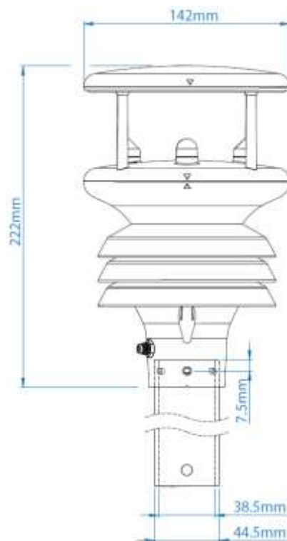
GMX550
