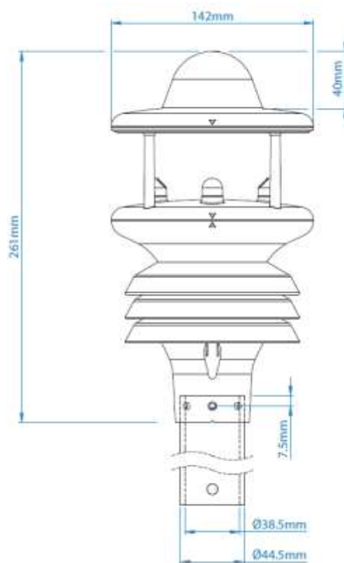
GMX600
