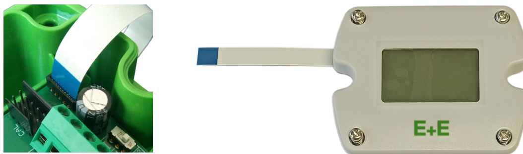
Fig. 9 Display and FFC cable connection on the EE210 electronics board
