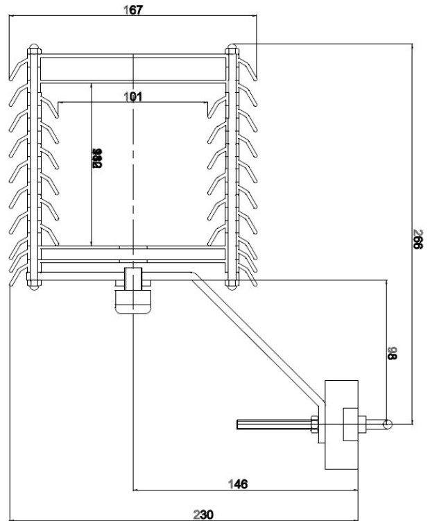
OMC-422 dimensions
