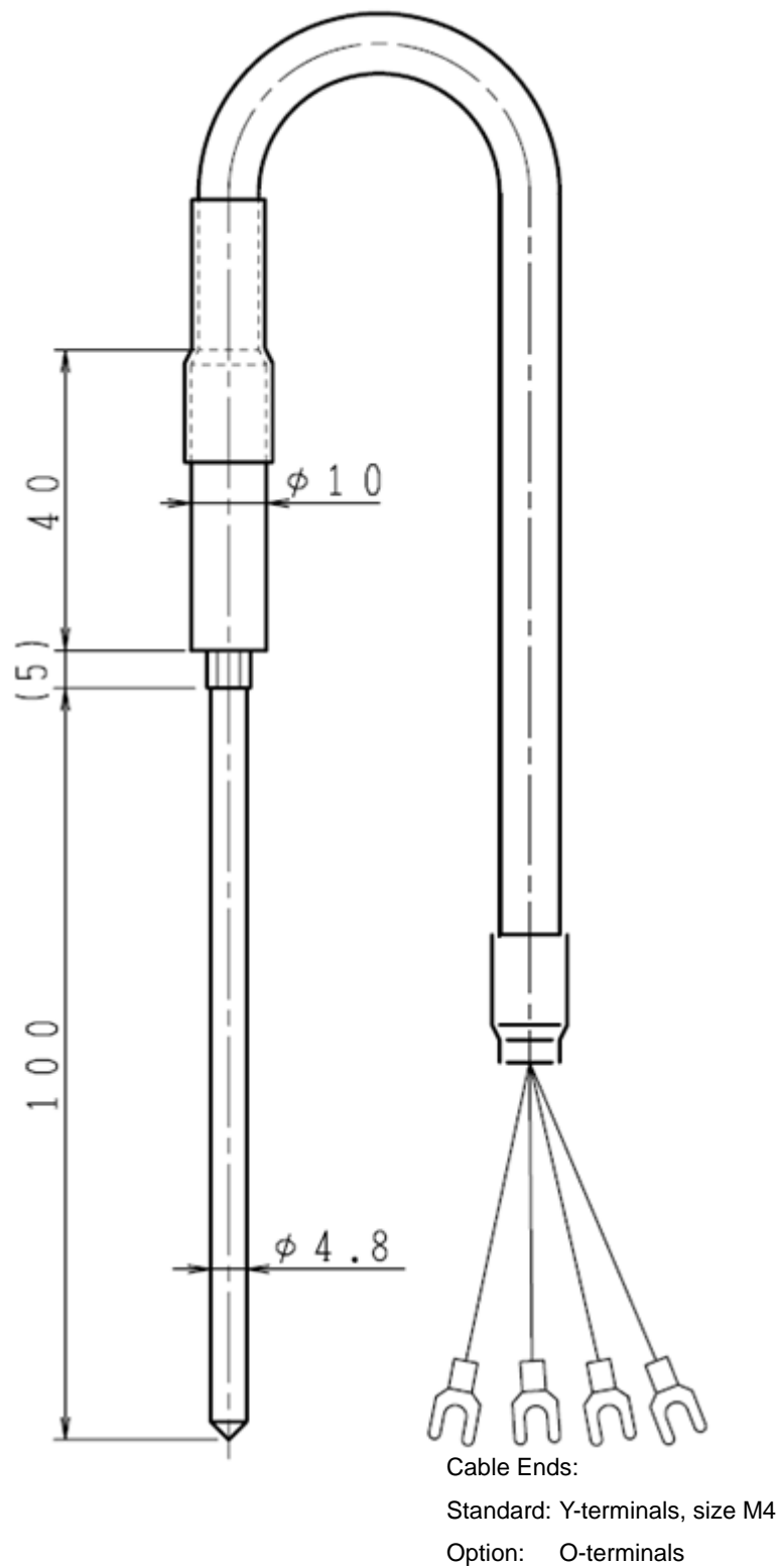
Figure 6-2. MT-010 Temperature Sensor Dimensions
