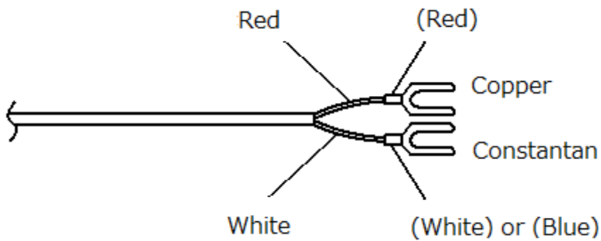
Figure 4-16. MT-052-T Wiring
