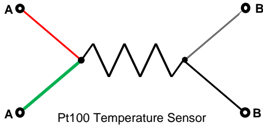
Figure 4-12. Circuit Diagram of the PT100 Temperature Sensor
