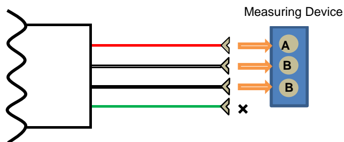
Figure 4-14. 3-wire Connection
