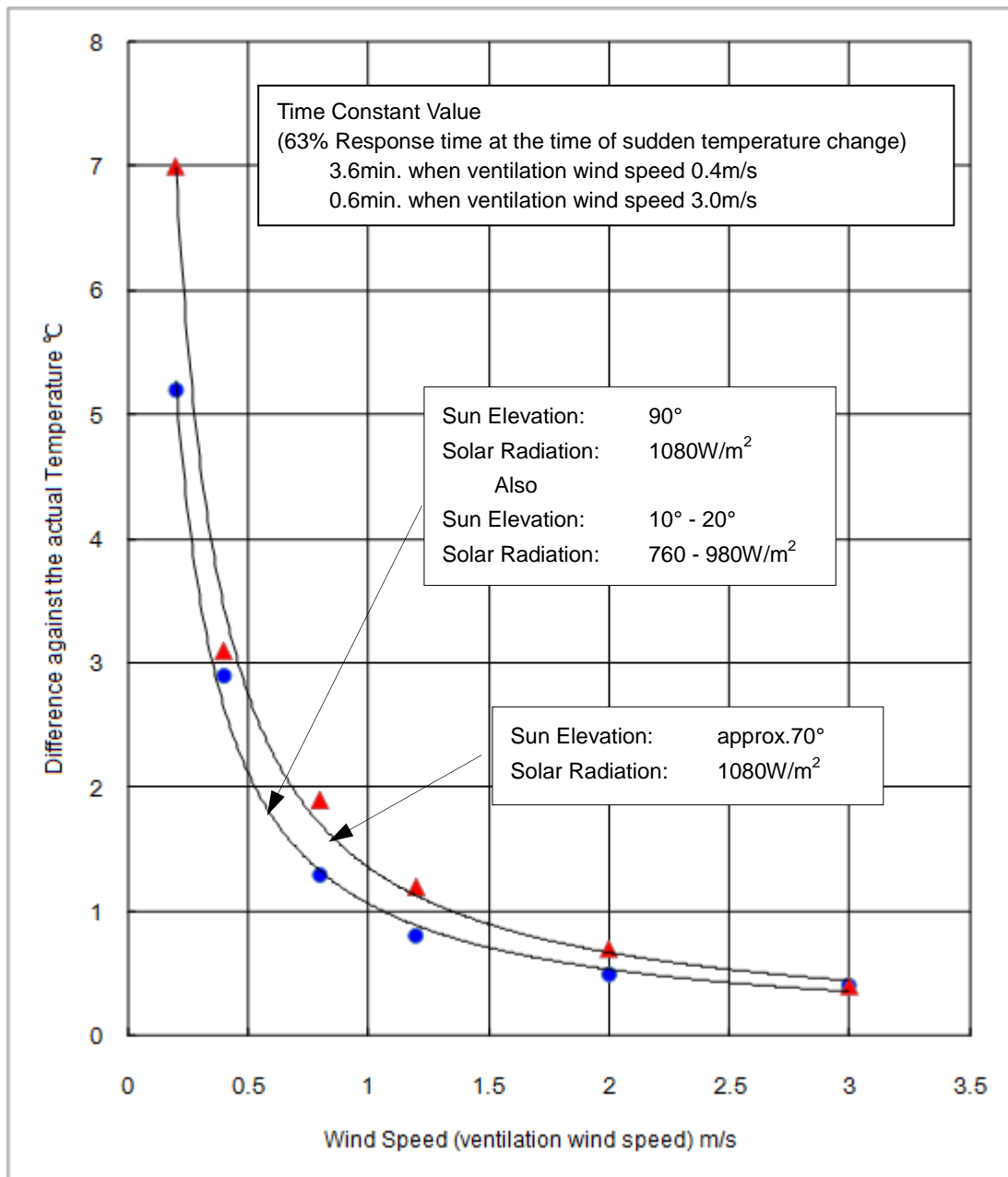
Figure A-1. Wind speed and Sun Elevation Effects on Temperature inside MT-052-A
