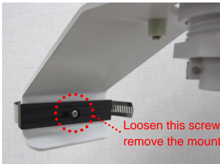
Figure 4-9. Back side of the Mounting Part
