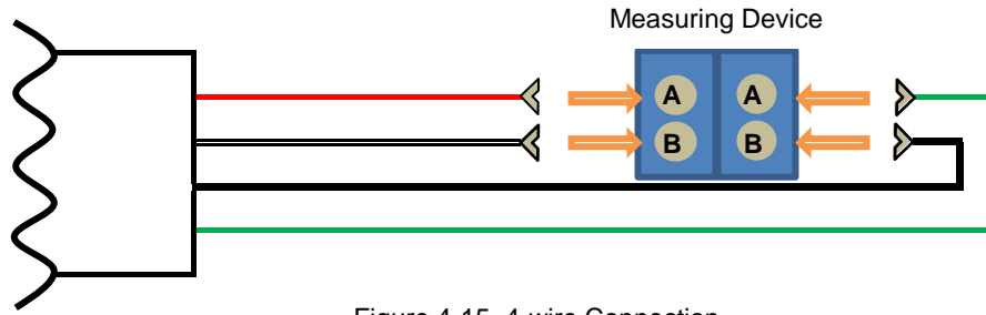
Figure 4-15. 4-wire Connection
