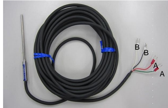
Figure 4-13. Wiring Colors
