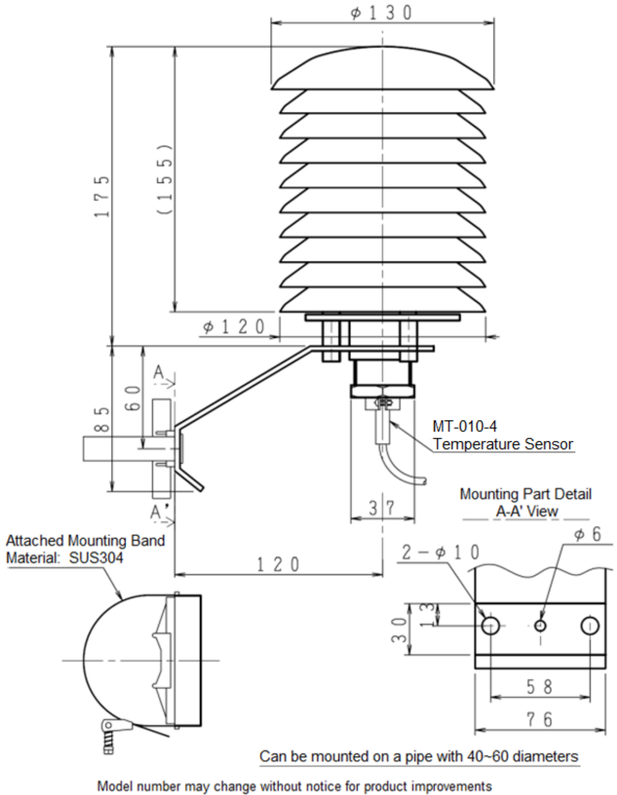
Figure 6-1. Radiation Shield Dimensions
